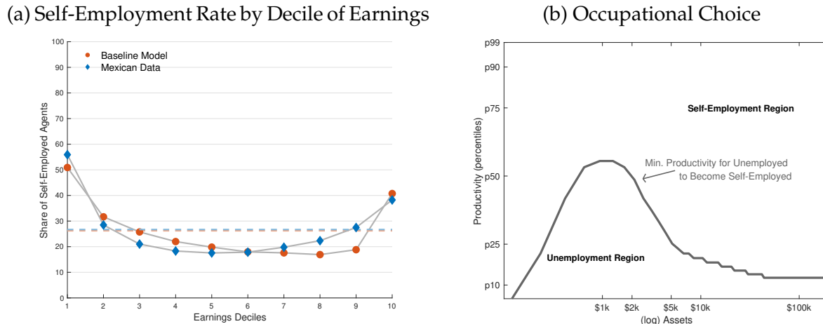
Figure 2: Model Performance
